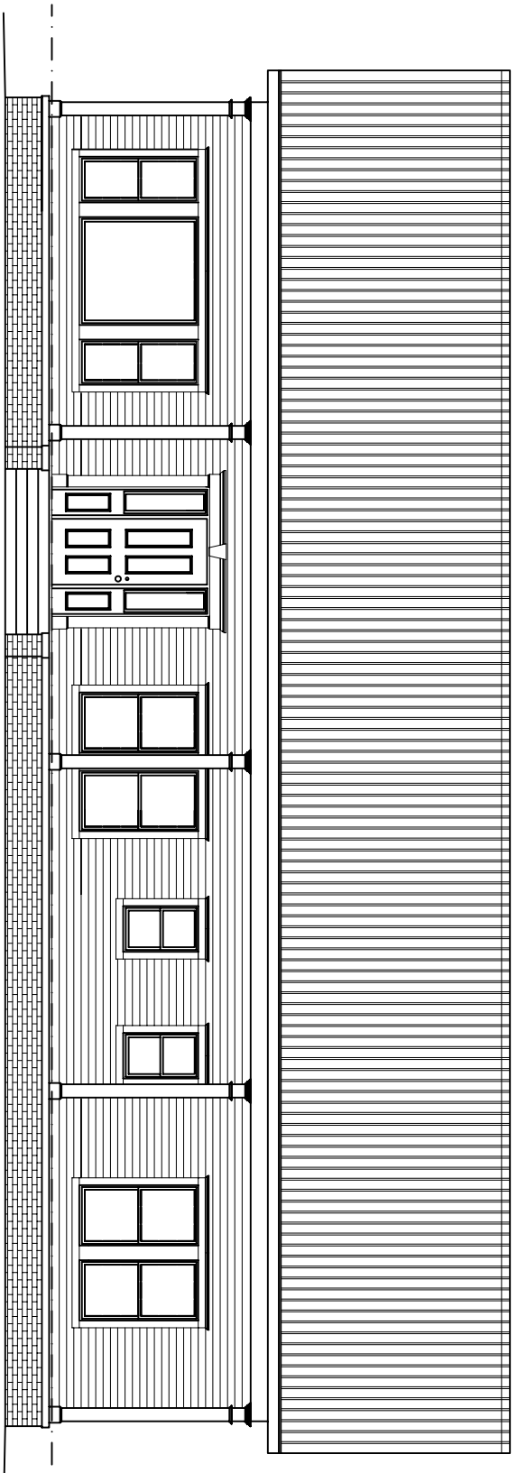
FRONT SIDEWALL ELEVATION 1/8"=1'-0"
