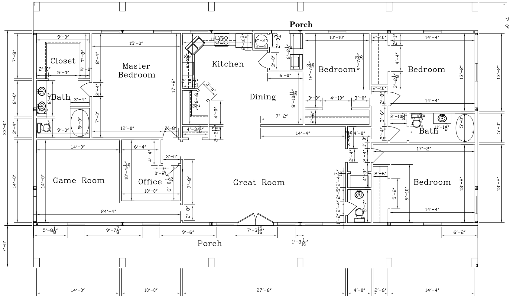
Hillcrest 7 Floor Plan 33' x 75' Living Area (2475 Square Feet) 7' x 75' Front and Rear Porch (1050 Square Feet)
