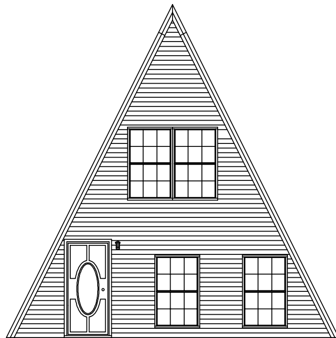
BACK SIDEWALL ELEVATION
