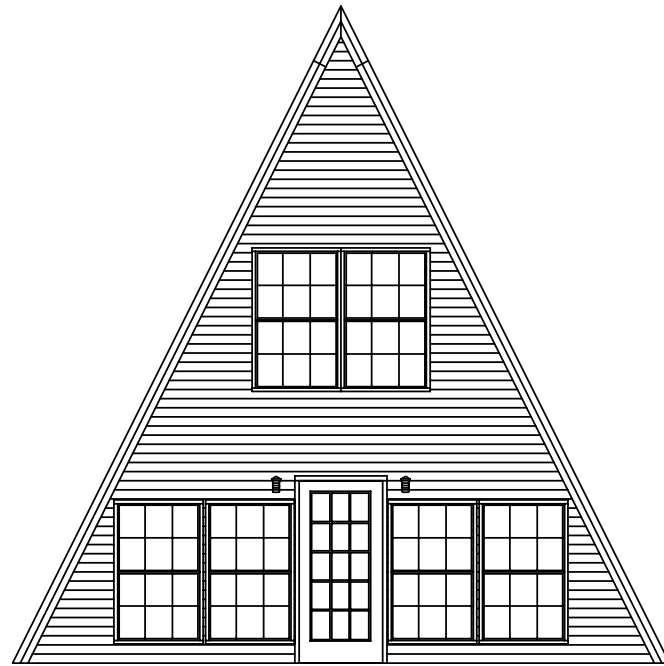
FRONT SIDEWALL ELEVATION
