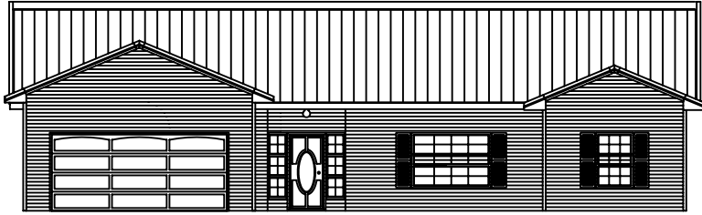
FRONT SIDEWALL ELEVATION
