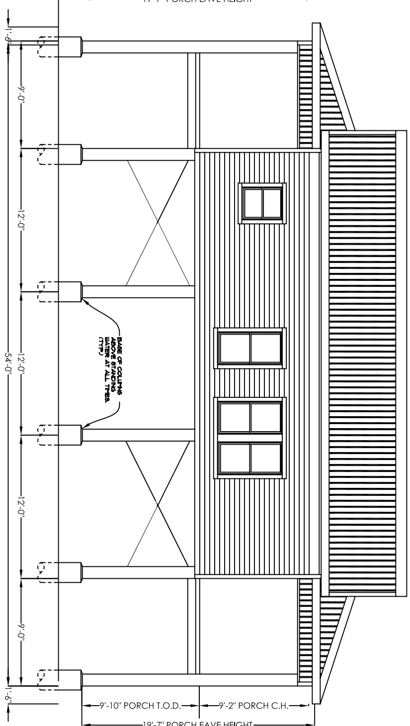
LEFT SIDE ELEVATION 1/8"=1'-0"
