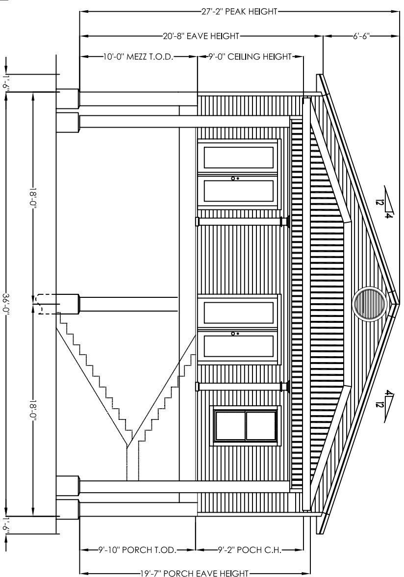
REAR ELEVATION 1/8"=1'-0"
