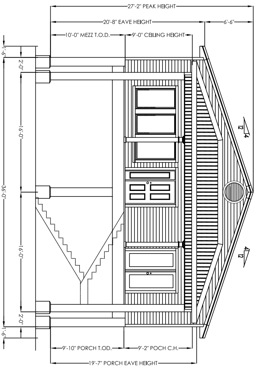
FRONT ELEVATION 1/8"=1'-0"
