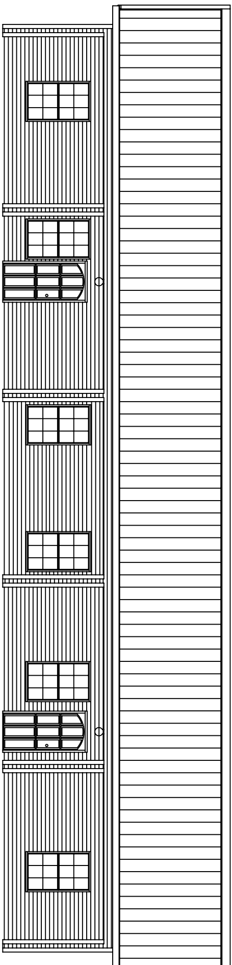
FRONT SIDEWALL ELEVATION
