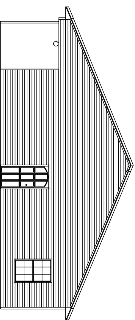
RIGHT ENDWALL ELEVATION
